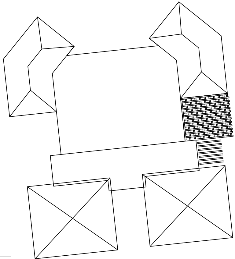
Roof Plan
